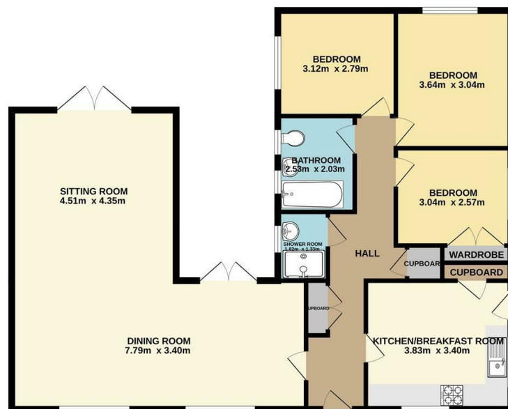
GROUND FLOOR 108.5 sq.m. approx.
